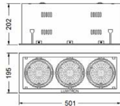
LMDL-182-3 Cut-out 464x164 mm
