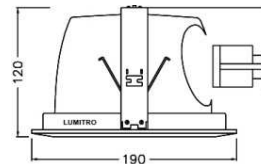
LMDL-5C Cut-out 178mm
