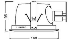
LMDL-5B Cut-out 150mm
