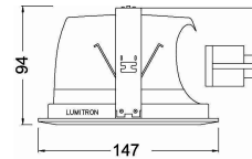
LMDL-5A Cut-out 120mm
