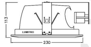
LMDL-5D Cut-out 215mm
